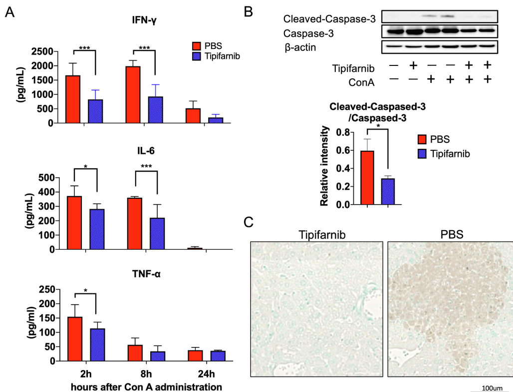
Fig. 2. The effect of tipifarnib on cytokine increments induced by Con A. (A) The serum protein-expression levels of IFN- \gamma , IL-6, and TNF- \alpha were quantified by ELISA at 2, 8, and 24 h after Con A administration ( N = 6 in each group). (B) Representative immunoblots and densitometric analysis of cleaved caspase 3. The expression levels of cleaved caspase 24 h after Con A administration. Relative intensity was normalized to uncleaved caspase 3 expression levels ( N = 6 ). (C) The liver section stained by TUNEL assay. The data shown are expressed as the mean ± SEM. * p < 0.05 , *** p < 0.001 between the PBS and tipifarnib groups. Red columns, PBS group. Blue columns, tipifarnib group. Scale bars, 100 \mu m. (For interpretation of the references to color in this figure legend, the reader is referred to the web version of this article.)
