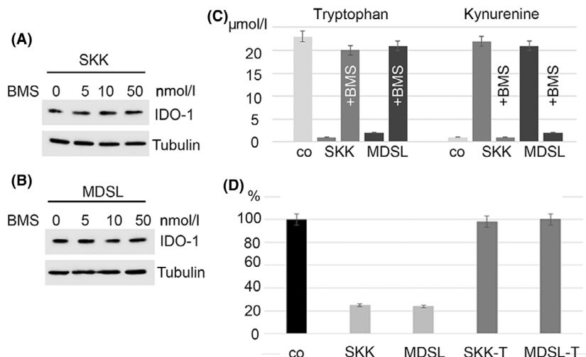
Fig 5. Tryptophan metabolism by MDS cell lines and inhibition of T cell proliferation. Western blot analysis of SKK (A) and MDS-L (B) cell lines display constant high expression of IDO-1 under BMS-986205 treatment in various concentrations (0–50 nmol/l). Tryptophan is catabolised in conditioned medium of SKK and MDS-L; simultaneously, kynurenine levels are increasing as measured by ELISA (C). MTT assays (D) show a clear reduction of T cell proliferation in conditioned medium (SKK, MDS-L), which can be rescued by addition of tryptophan (SKK-T, MDS-L-T).
