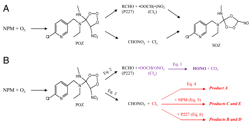
Fig. 1. (A) Conventional mechanism of ozonolysis applied to NPM; (B) abbreviated proposed mechanism consistent with observed products. Detailed proposed mechanisms for formation of products A to E are found in SI Appendix , Figs. S7–S11.
